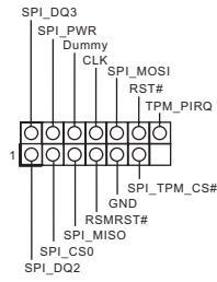
SPI_TPM_J1
